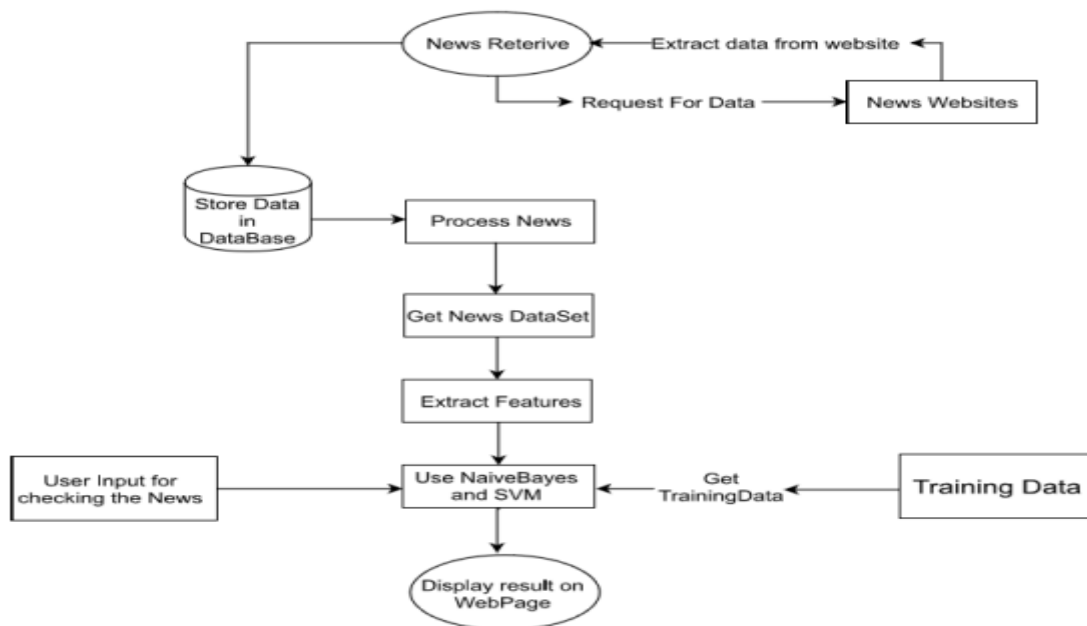
Figure 4.4 Flow chart – Proposed Model
