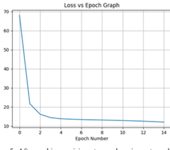
Figure 5. After making revisions to our learning rate and model input, we found that we found we had a consistently decreasing loss.
